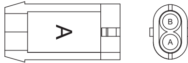
HB-3 Male Plug
