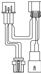
Adapter Kit HB-5 to HB-2 (PN 28860-1)
